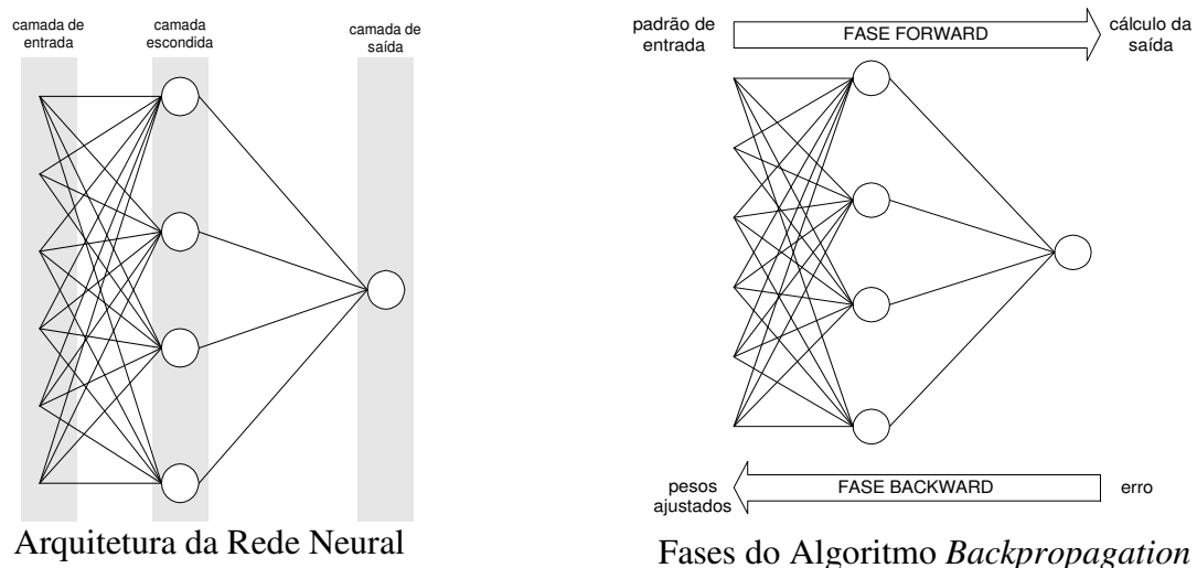
Figura 1 - Rede Multi Layer Perceptron .
